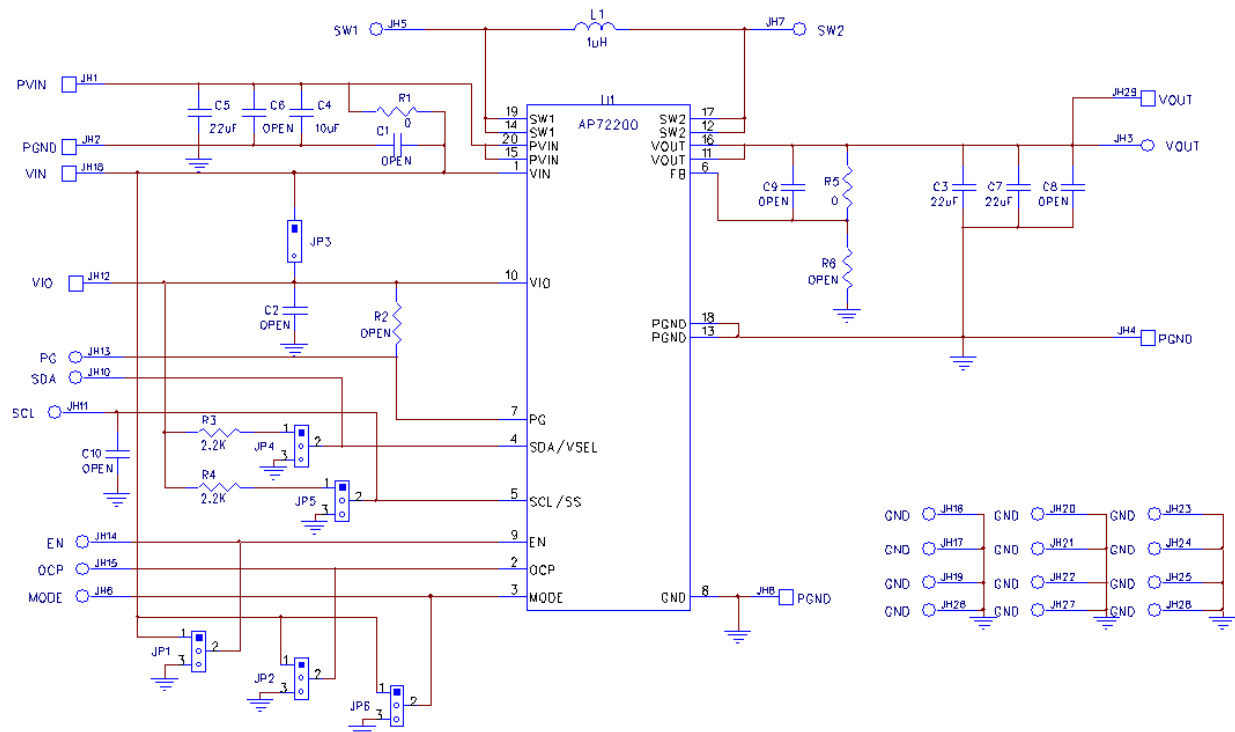
Figure 2. AP72200WLCSP-20-EVM Schematics
