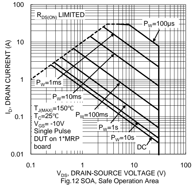
Fig. 12 SOA, Safe Operation Area
