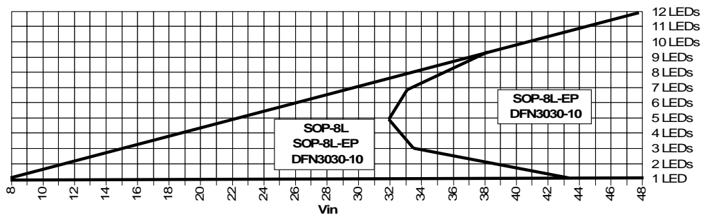
Figure 10: Suggested package for a 700mA application
