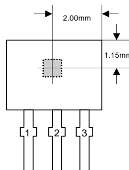
Sensor Location
