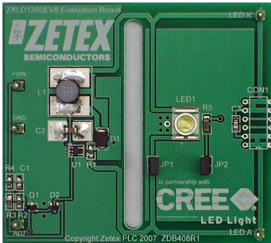
Figure 1: ZXLD1360EV8 evaluation board
