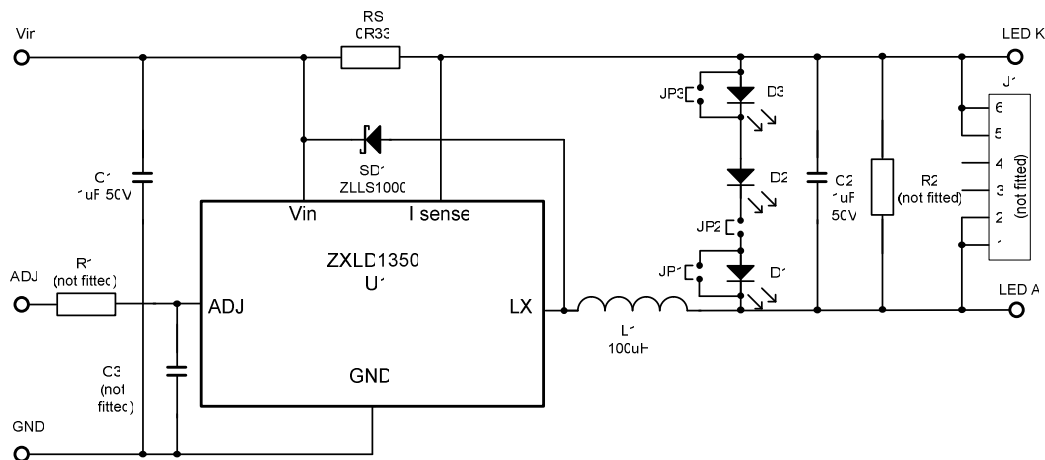
Figure 2: Schematic for the evaluation board ZXLD1350EV7
