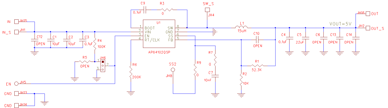
Figure 3. AP64102QSP-EVM Schematic
