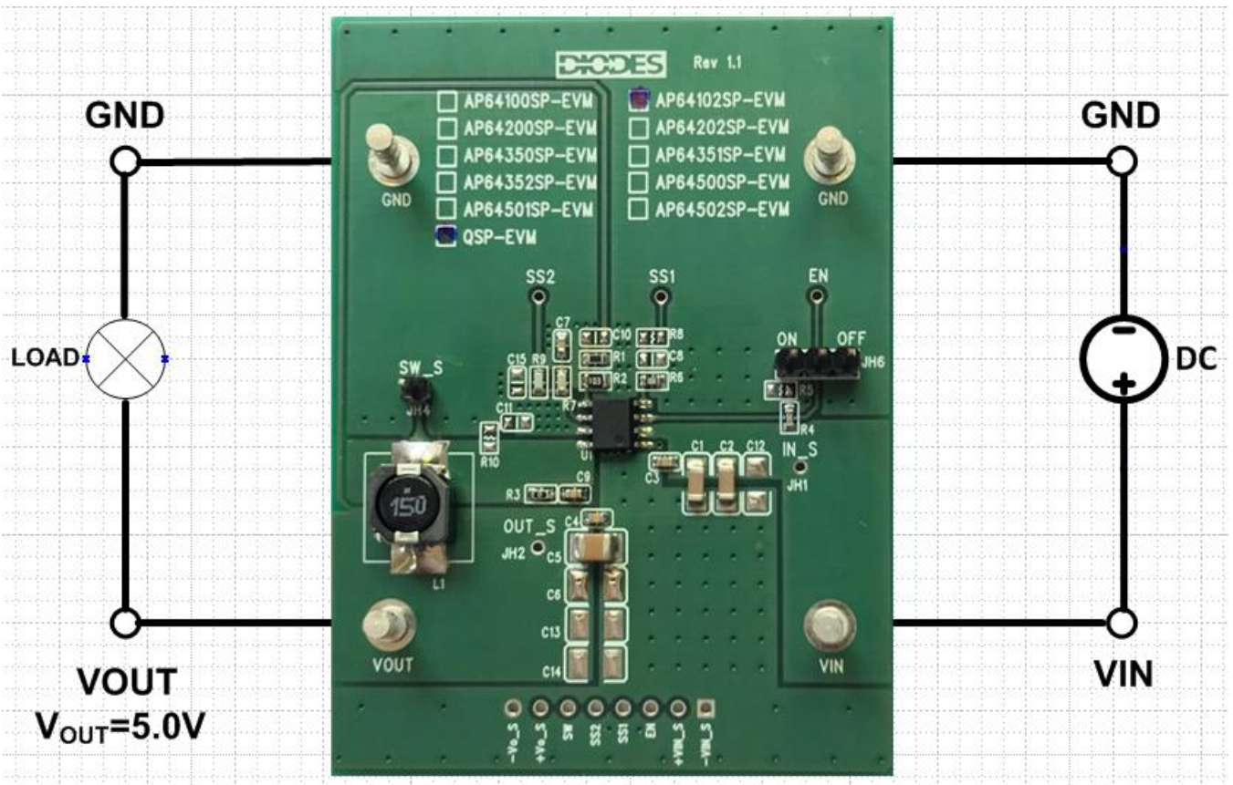
Figure 2. AP64102QSP-EVM
