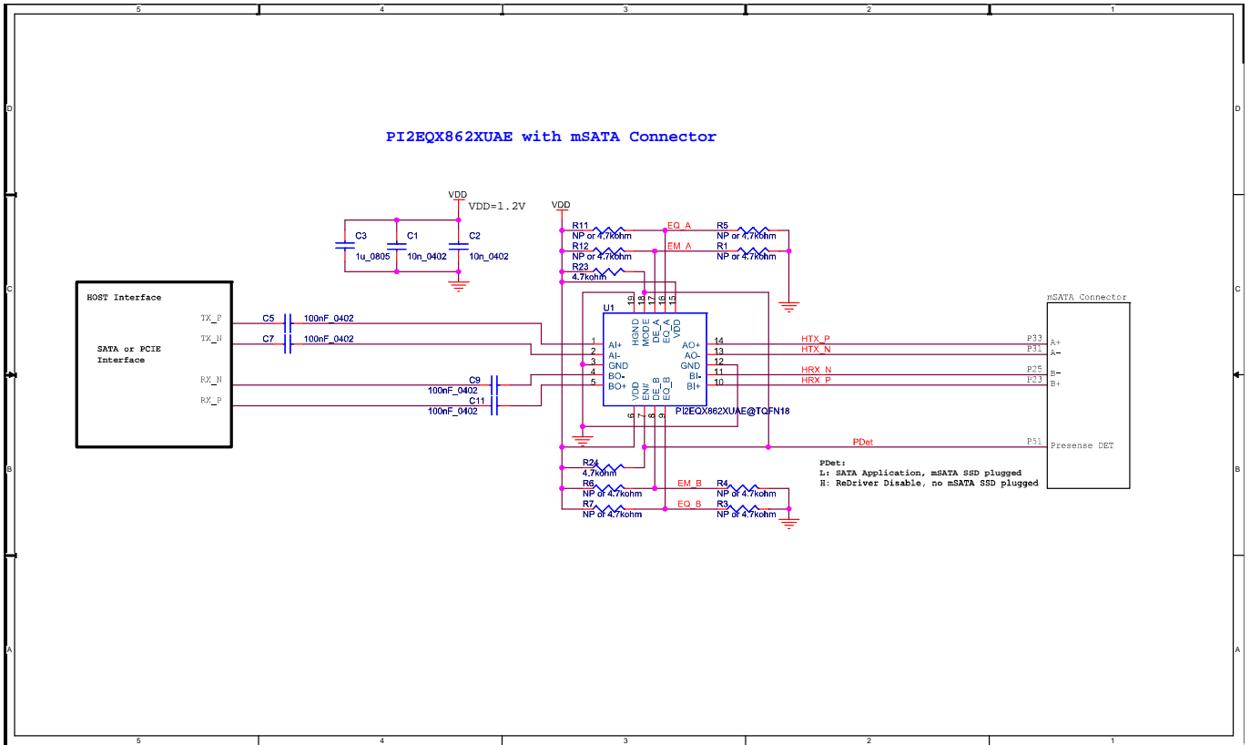
Figure 3: PI2EQX862XUAE with mSATA Connector
