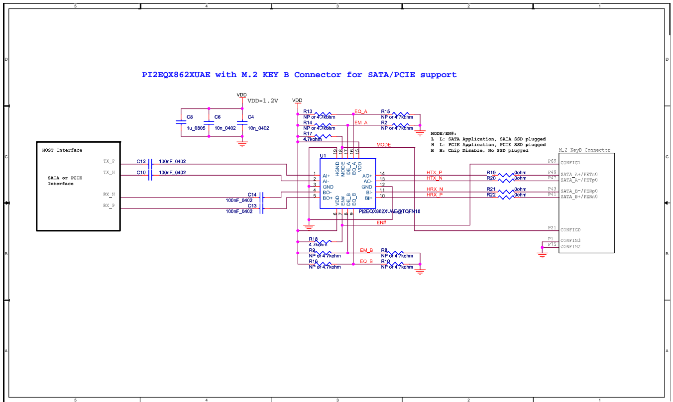
Figure 1: PI2EQX862XUAE with M.2 KEY B Connector for SATA/PCIE Support
