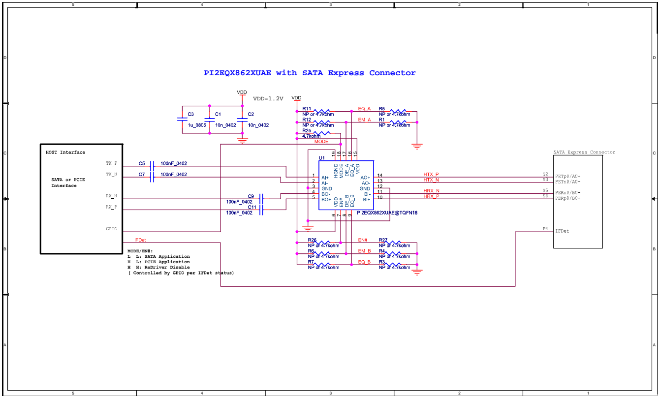
Figure 2: PI2EQX862XUAE with SATA Express Connector
