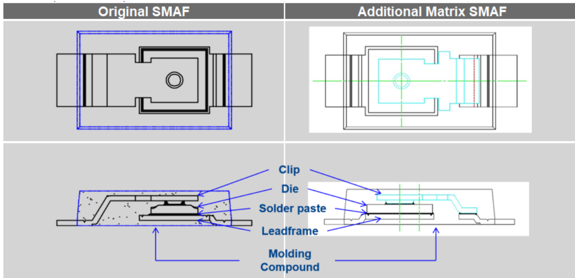
Figure 1: Comparison of SMAF (D-FLAT) Package Construction for SKY, GPP and TVS products
