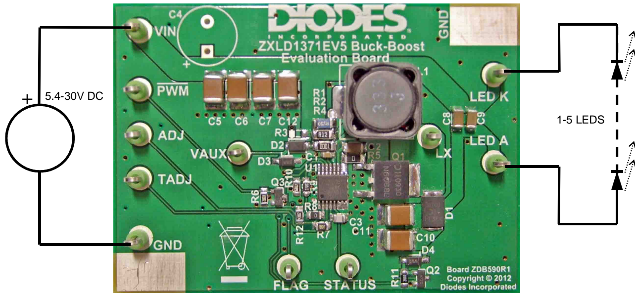
Figure 1: ZXLD1371EV5 evaluation board and connection diagram
