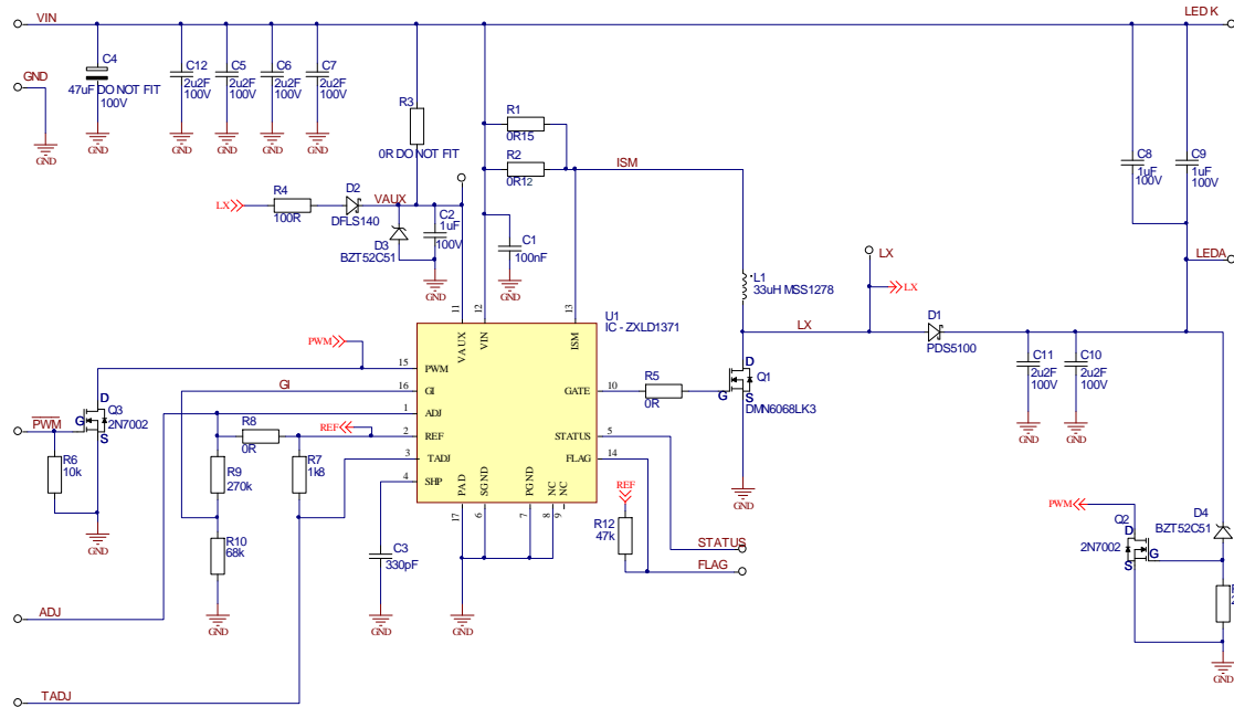
Figure 2: ZXLD1371EV5 evaluation board Schematic
