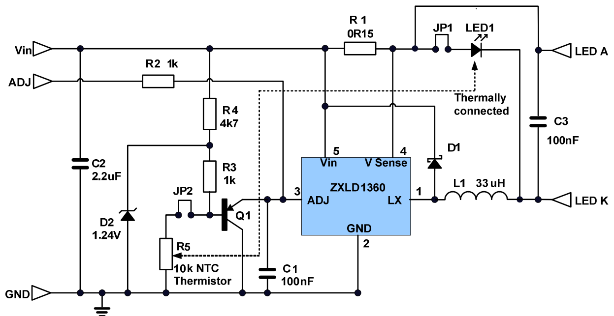
Figure 2: Schematic for the evaluation board ZXLD1360EV9
