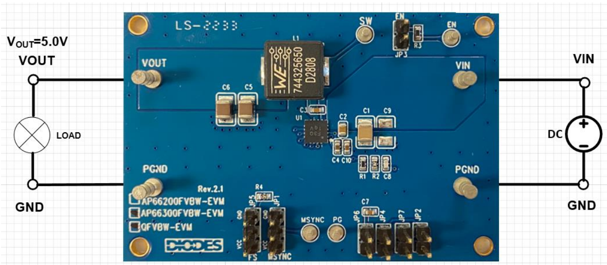
Figure 1. AP66300QFVBW-EVM
