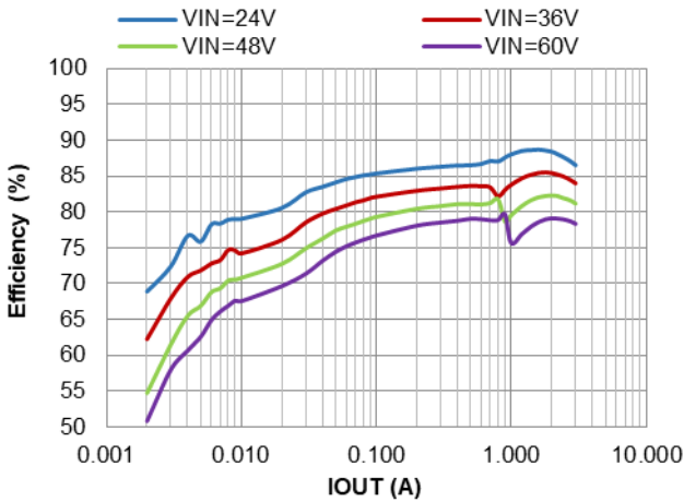
Figure 9. PFM Efficiency vs. IOU T, VOUT=3.3V, L=5.5µH
