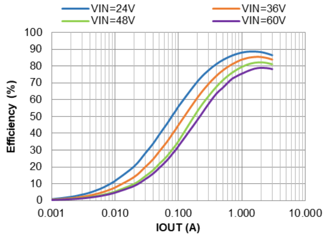
Figure 10. PWM Efficiency vs. IOU T, VOUT=3.3V, L=5.5µH
