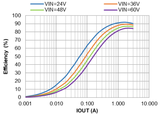
Figure 8. PWM Efficiency vs. IOU T, VOUT=5V, L=6.5µH
