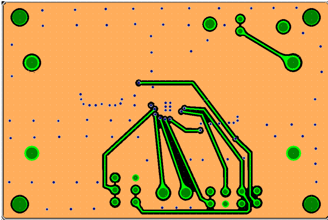
Figure 5. AP66300QFVBW-EVM – Layer 3
