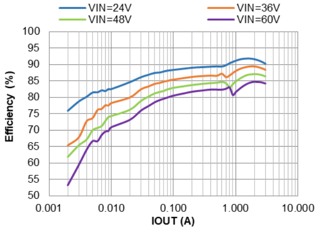
Figure 7. PFM Efficiency vs. IOU T, VOUT=5V, L=6.5µH
