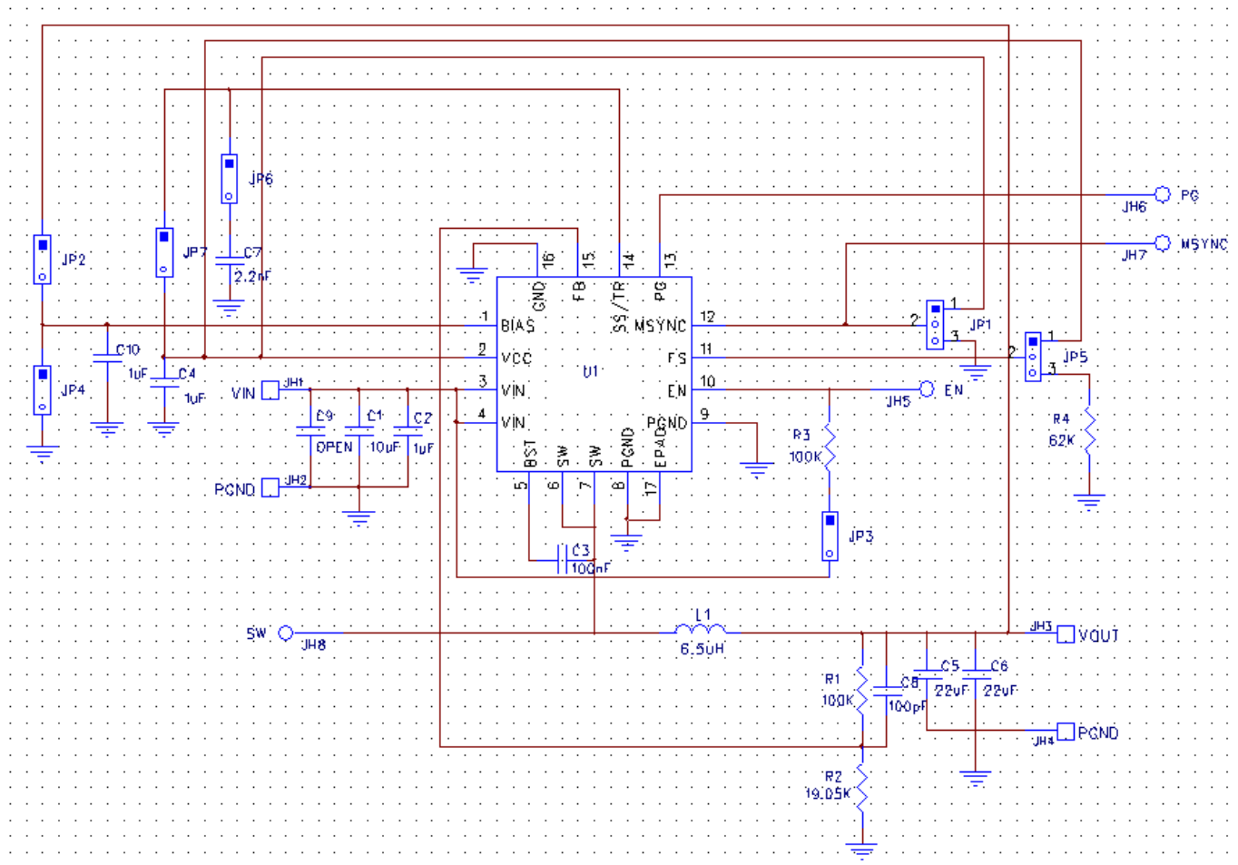
Figure 2. AP66300QFVBW-EVM Schematic
