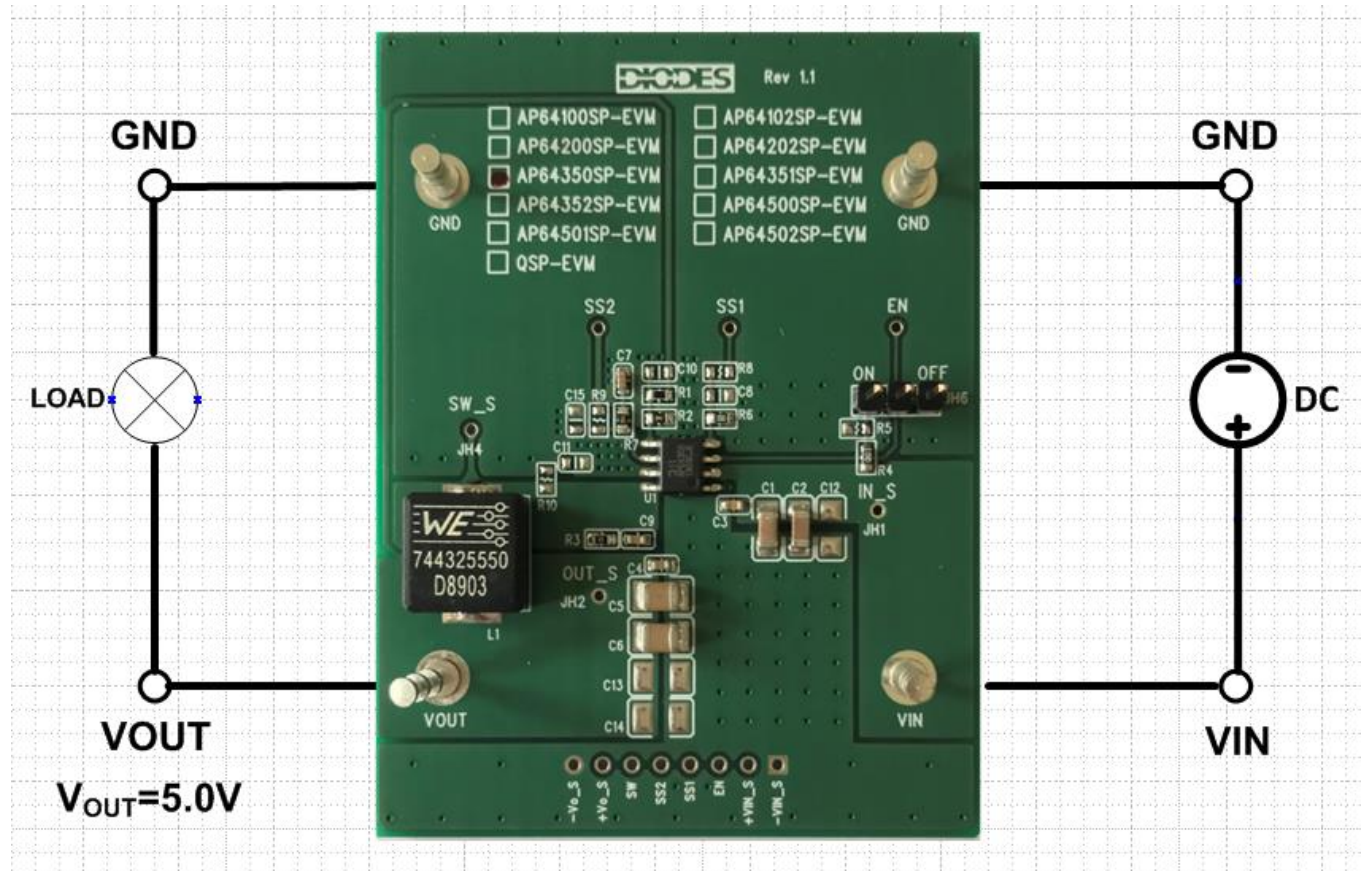
Figure 2. AP64350SP-EVM
