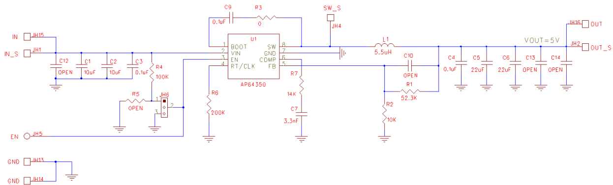
Figure 3. AP64350SP-EVM Schematic
