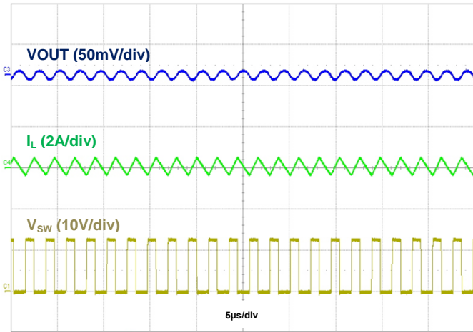
Figure 7. AP63356Q Output Voltage Ripple, VIN = 12V, VOUT = 5V, IOUT = 50mA
