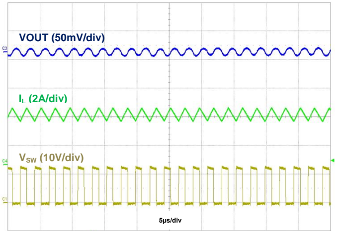
Figure 8. AP63356Q Output Voltage Ripple, VIN = 12V, VOUT = 5V, IOUT = 3.5A
