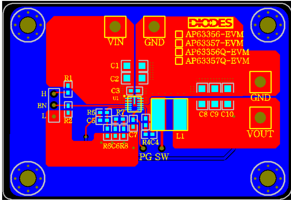
Figure 4. AP63356QZV-EVM – Top Layer
