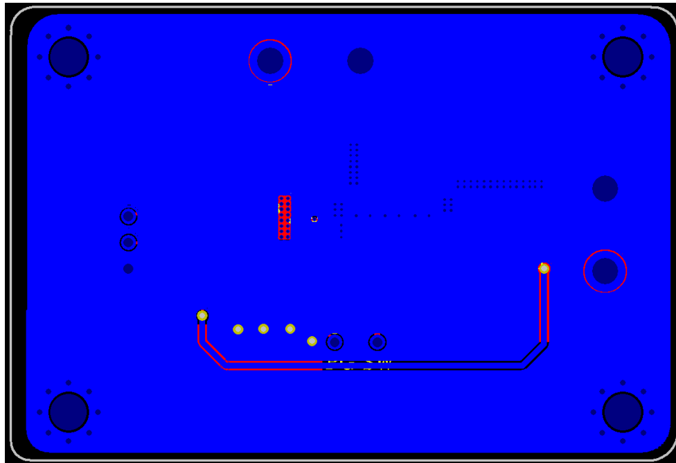
Figure 5. AP63356QZV-EVM – Bottom Layer
