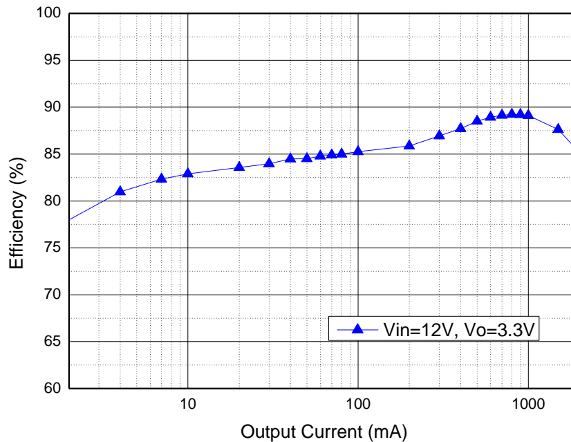
Figure 4. Efficiency for VIN=12V, VOUT= 3.3V
