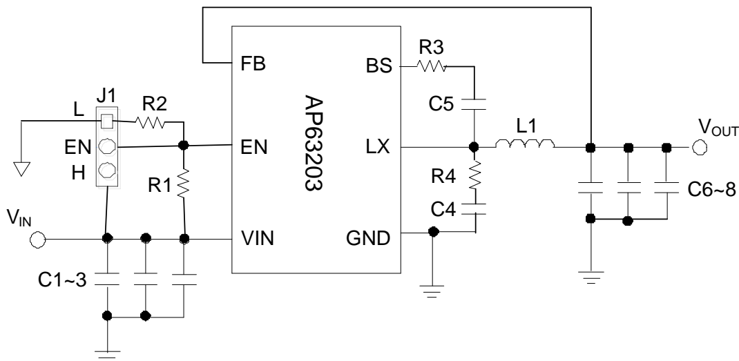
Figure 3. AP63203WU-EVM Schematic
