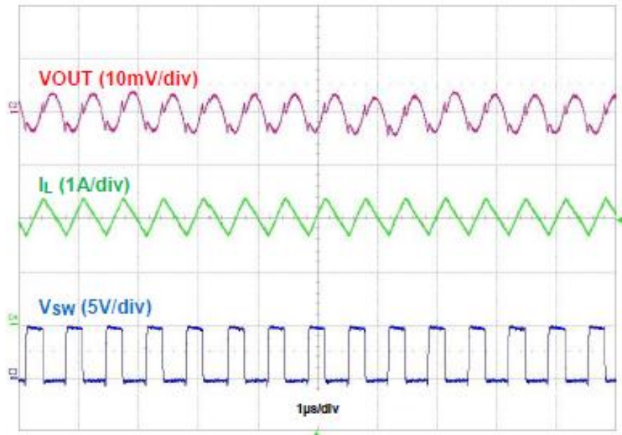
Figure 8. Output Voltage Ripple, IOU = 2A
