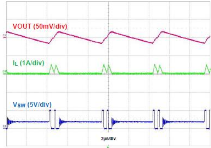
Figure 7. Output Voltage Ripple, IOU = 50mA
