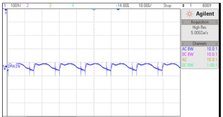
Figure:17 5V Ripple at 230Vac at FL
