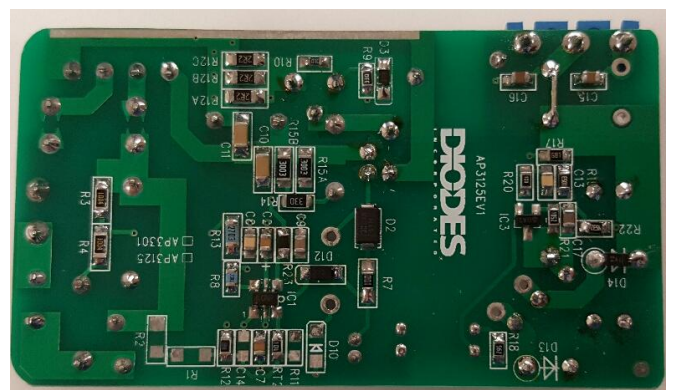
Figure 2: Bottom View
