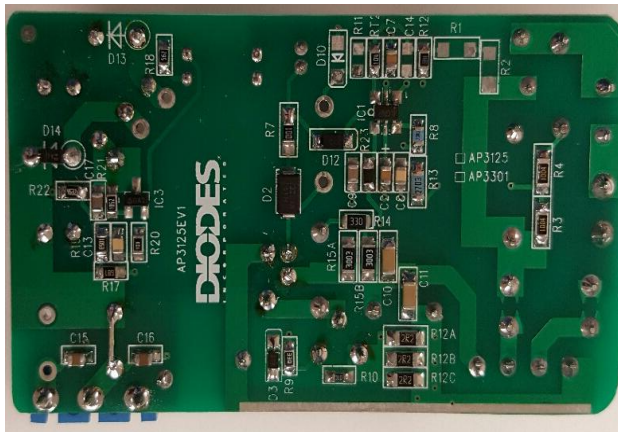
Figure:18 SMD components UP side
