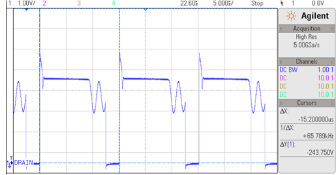
Fig:7 Vds at full load by using DF probe 1:100 at 230V AC
