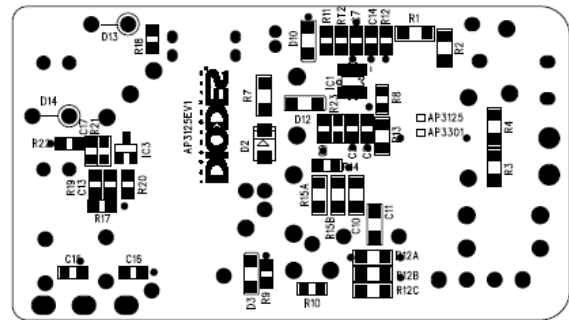
Figure 5: PCB Board Layout Bottom View
