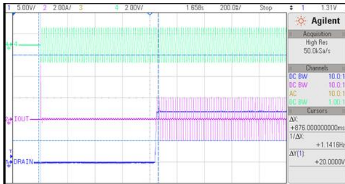
Fig:12 Turn on VAC_in, IAC_in, 12Vo at 115Vac at FL
