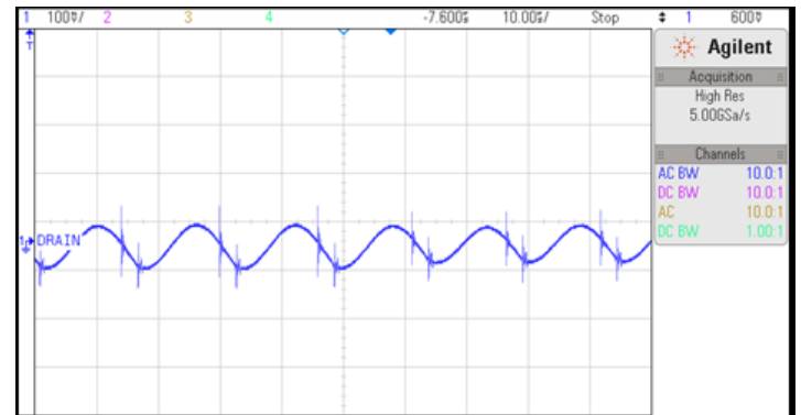
Figure:15 12V Ripple at 230Vac at FL
