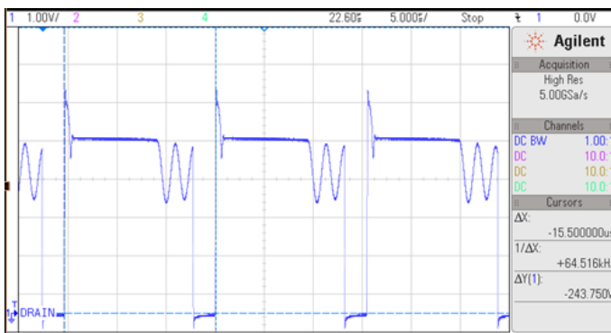
Fig:8 Vds at full load using DF probe 1:100 at 265V AC
