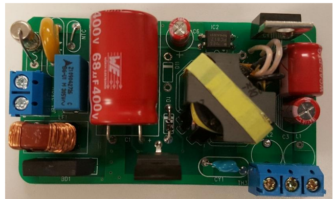
Figure 1: Top View
