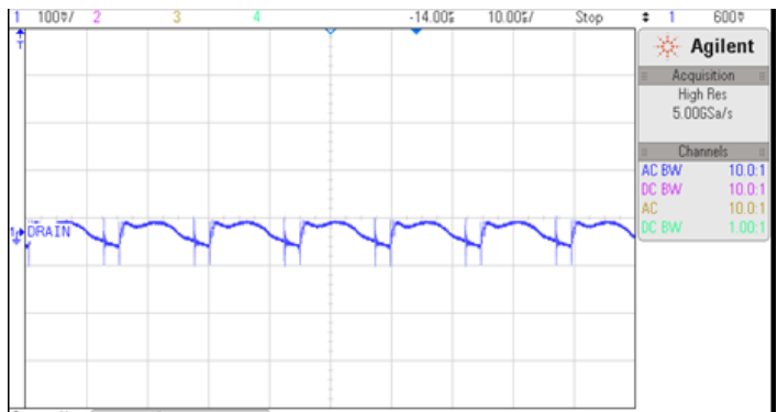
Figure:16 5Vo Ripple at 115Vac at FL
