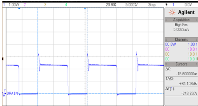
Fig:6 Vds at full load by using DF probe 1:100 at 115V AC
