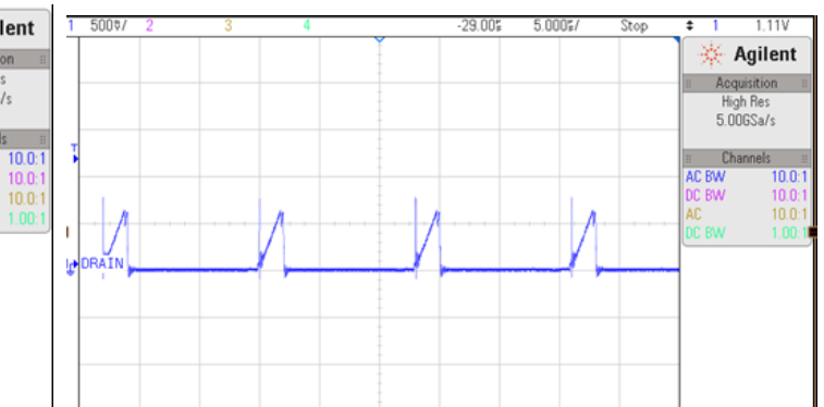
Fig:11 Vcs at 264V ACin at FL
