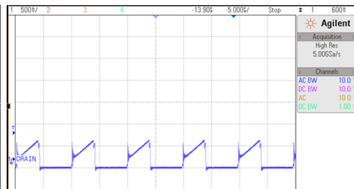
Fig:9 Vcs at 90V ACin at FL
