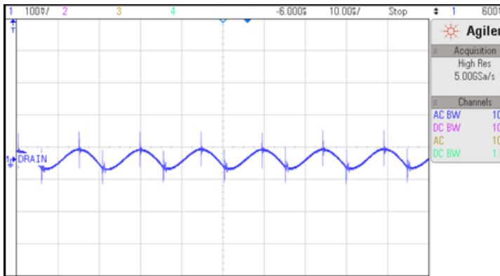
Figure:14 12V Ripple at 115Vac at FL .
