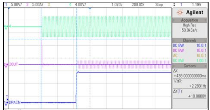
Fig:13 Turn on VAC_in, IAC_in, 12Vo at 230Vac at FL
