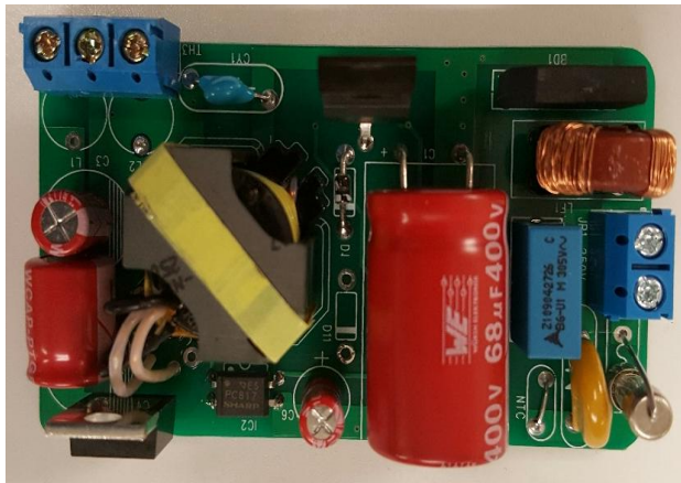
Figure:20 Board Top components side
