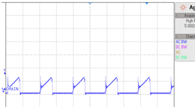
Fig:10 Vcs at 115V ACin at FL
