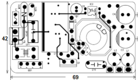
Figure 4: PCB Board Layout Top View
