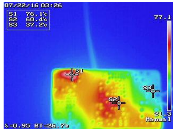
Figure:19 SMD side Vin=115V AC , Test time=1hour
