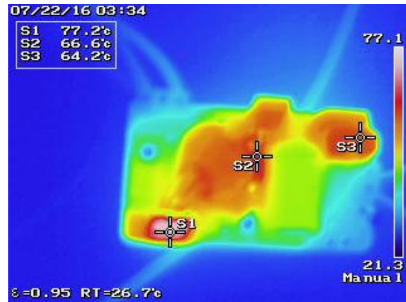
Figure:21 Vin=115V AC , Testing time = 1.15 hour
