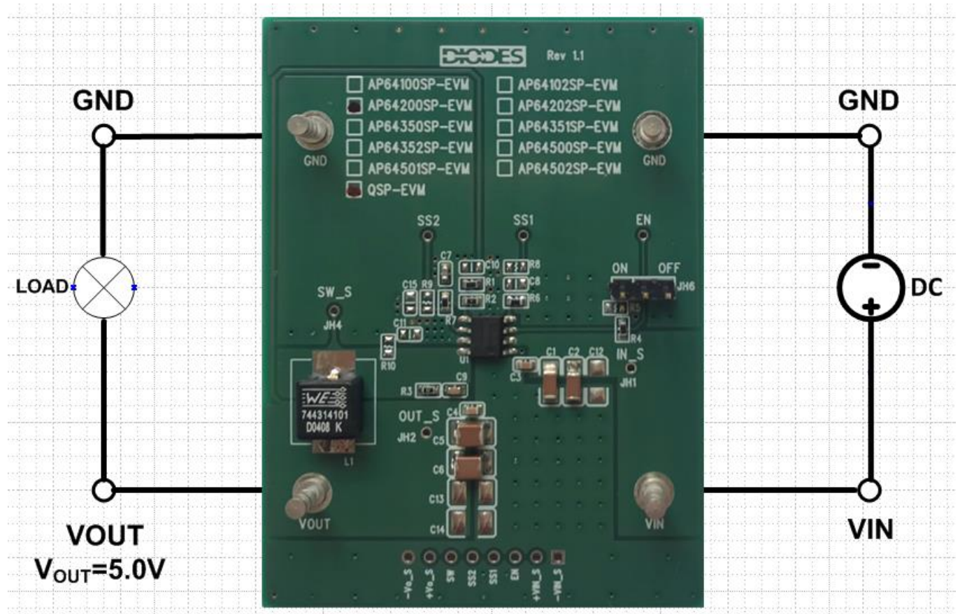
Figure 2. AP64200QSP-EVM
