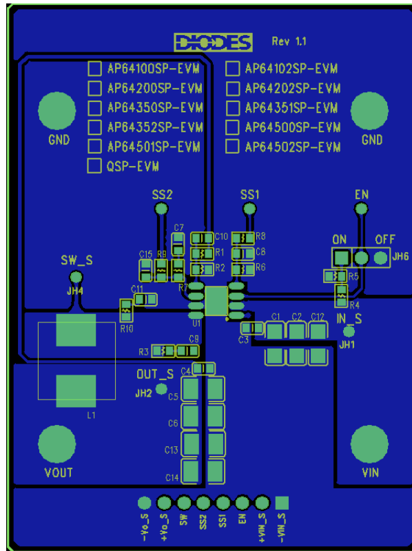
Figure 4. AP64200QSP-EVM – Top Layer
