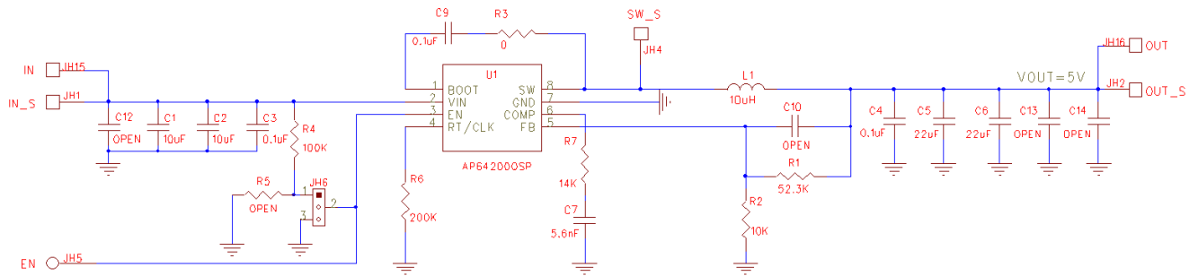
Figure 3. AP64200QSP-EVM Schematic
