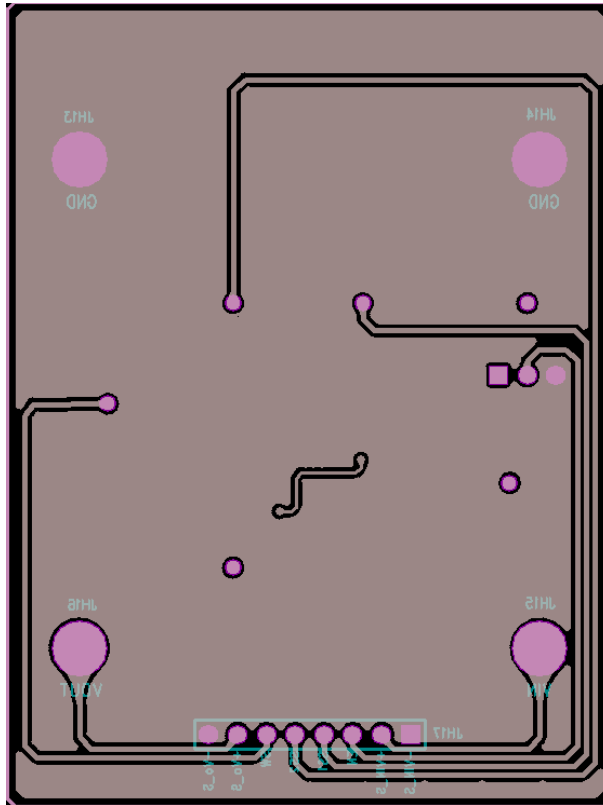
Figure 5. AP64200QSP-EVM – Bottom Layer
